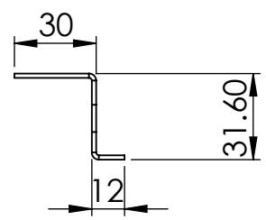
DETAIL L SCALE 2 : 5
